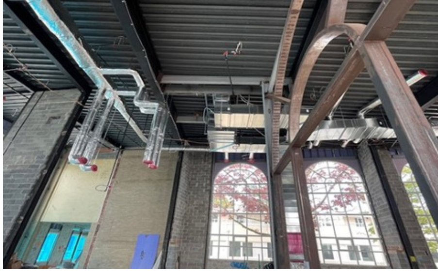
Chapel ceiling mechanical work in progress
