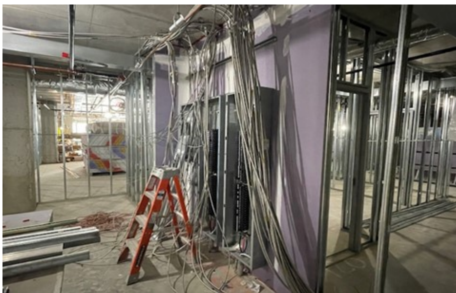
Electrical rough-in work in progress
